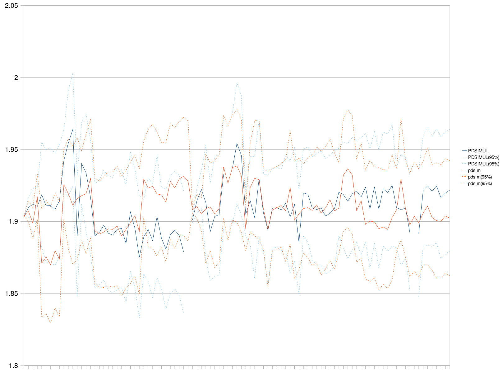
Mean Trait Value at 96 nodes form 10,000 runs of PDSIMUL and pdsim with 95% confidence intervals.
